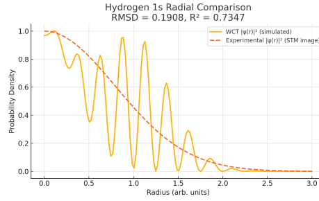
Figure 17: Simulated hydrogen |\psi(r)|^2 density (WCT) compared to experimental STM data.
