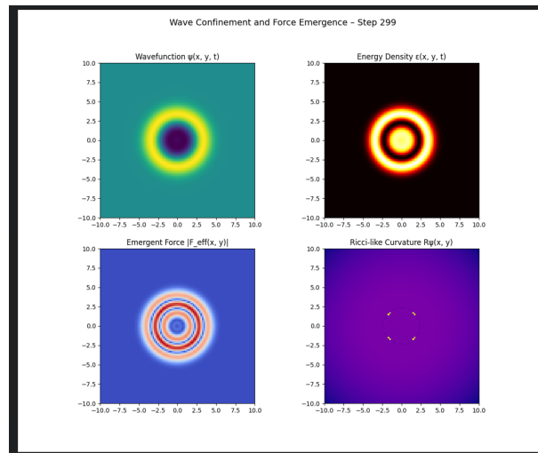
Figure 21: Wave Confinement
