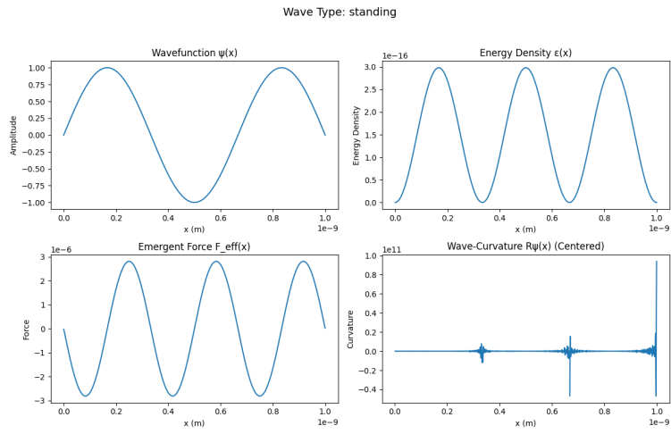
Figure 27: Standing
