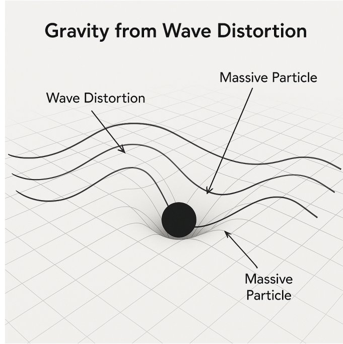
Figure 2: Gravity Well
