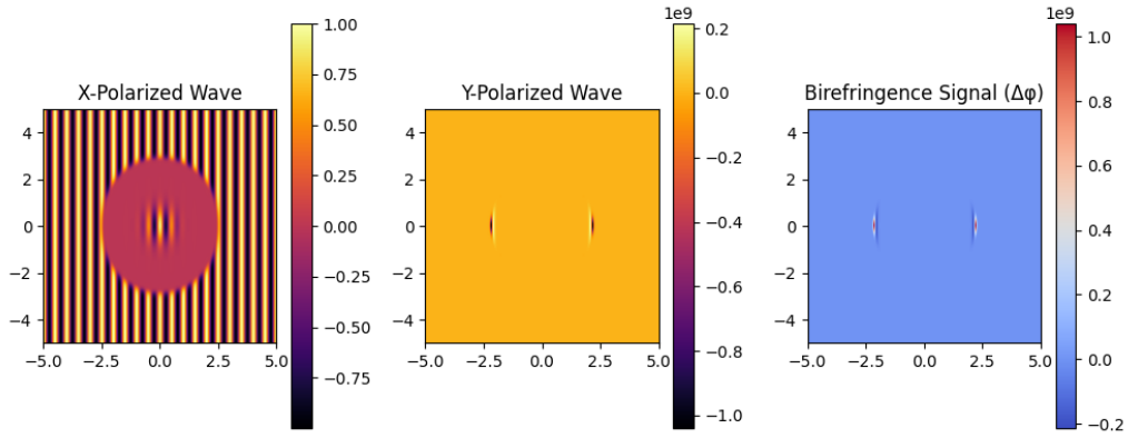
Figure 25: Emergent vacuum birefringence in WCT. (Left) X-polarized wave E_x is attenuated in high-gradient regions. (Center) Y-polarized wave E_y is enhanced. (Right) Their difference \Delta\phi shows spontaneous anisotropy of the confined vacuum.
