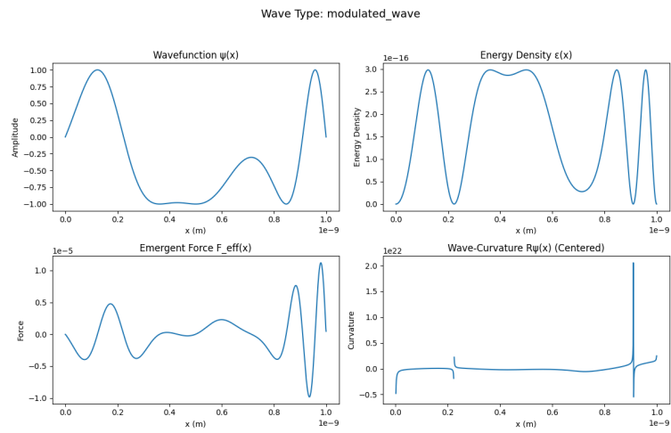
Figure 26: Modulated Wave
