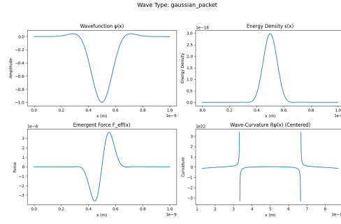
Figure 6: Gaussian Packet
