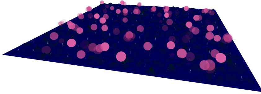
Figure 5: Wave Confinement Simulation
