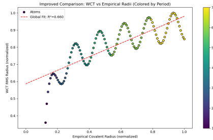
Figure 16: Normalized WCT RMS radii vs. empirical covalent radii, colored by atomic period.
