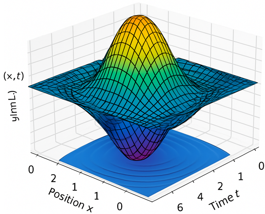
Figure 20: Rotating 3D Wave Packet Curved Spacetime
