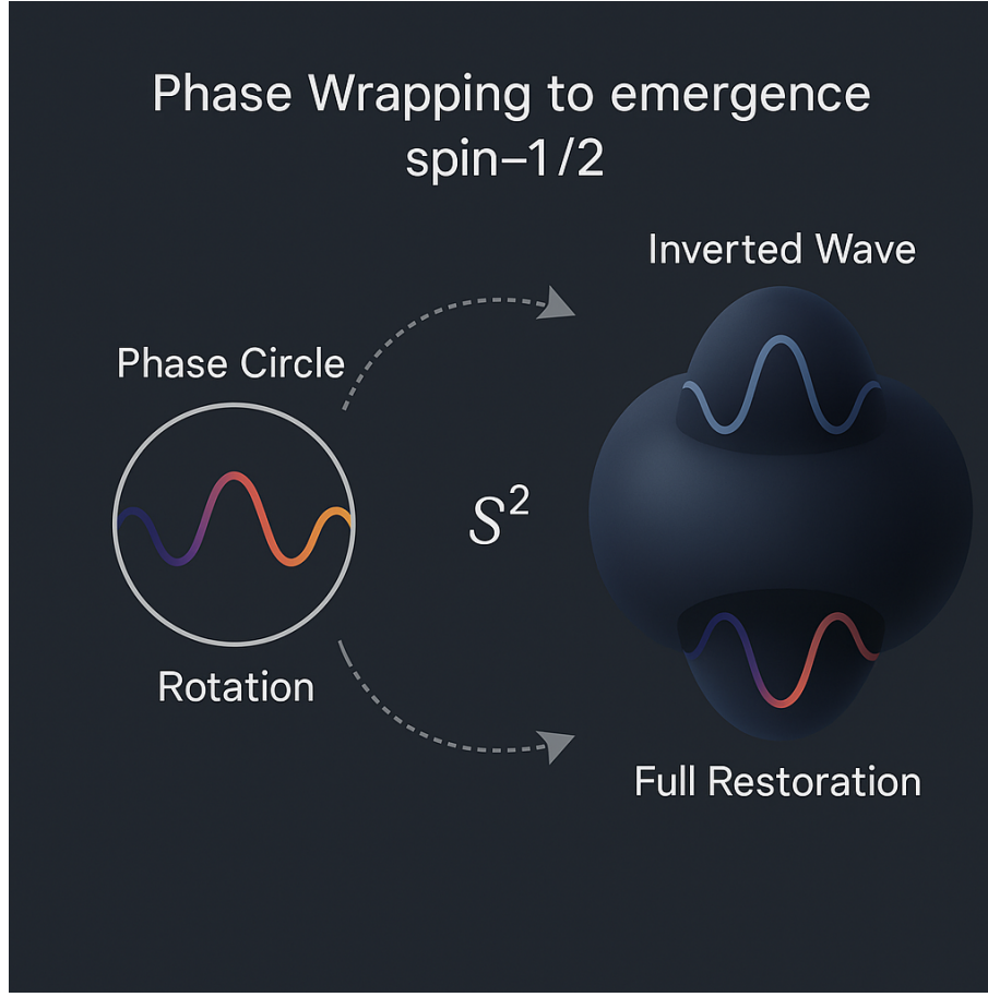
Figure 13: U(1) S(2) S(3) Example
