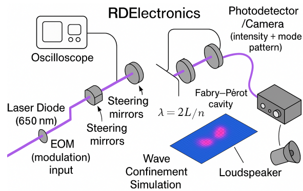
Figure 22: Wave Confinement Laser Experiment
