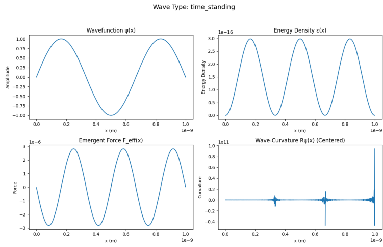
Figure 29: Time Standing
