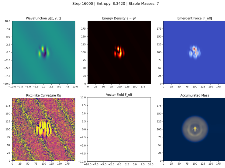
Figure 12: Curvature-Confined Modes: Interference geometry generates local curvature wells.
