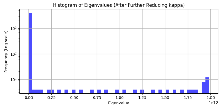
Figure 23: Eigenvalue Singularities Present
