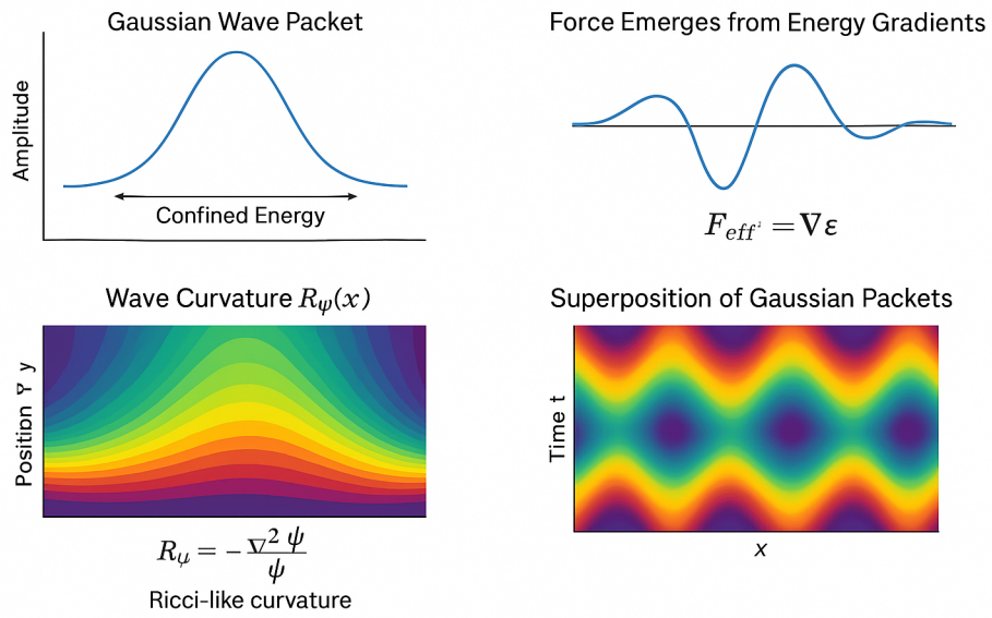
Figure 8: Gaussian Packet
