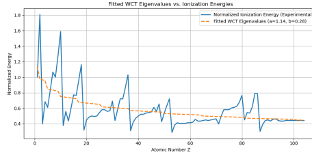
Figure 14: Fitted WCT eigenvalues compared to experimental ionization energies.
