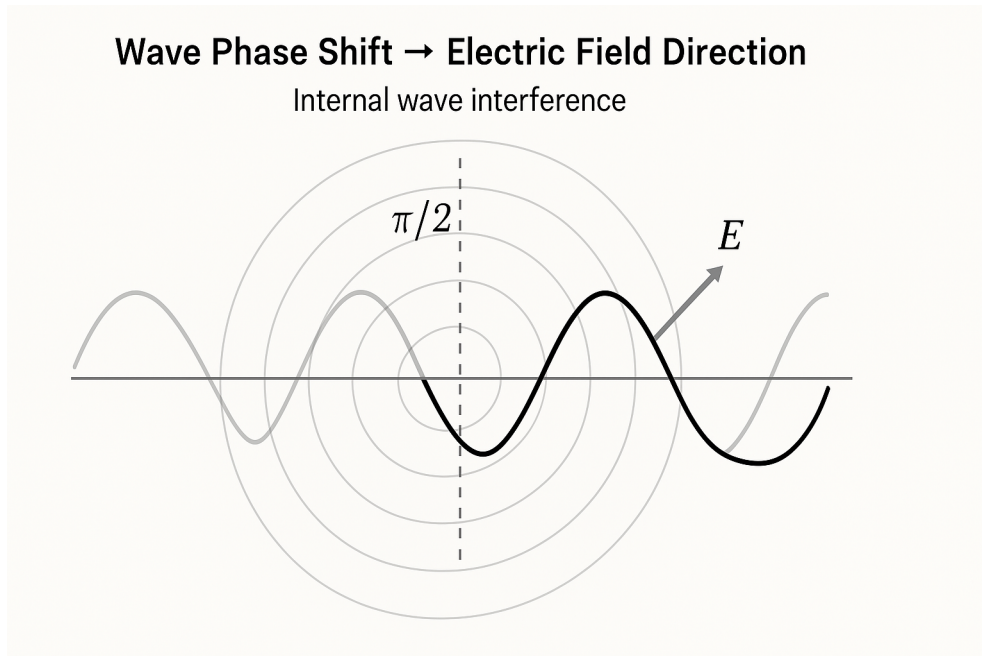
Figure 9: Phase Shift
