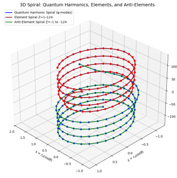
Figure 18: 3D spiral visualization of quantum harmonics, elements, and anti-elements.
