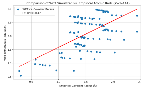
Figure 15: Raw WCT simulated RMS radii vs. empirical covalent radii.
